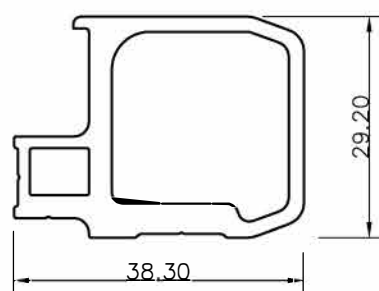
Ref. 35015SA
