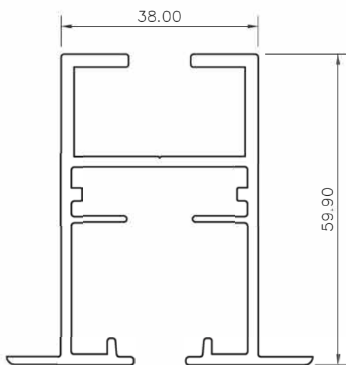
Ref. 35009***
