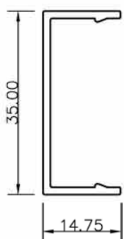
Ref. 35905**
