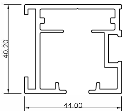
Ref. 35900**
