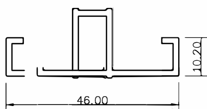
Ref. 35906**
