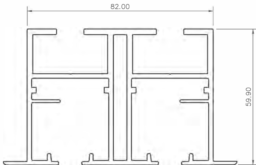
Ref. 35010***
