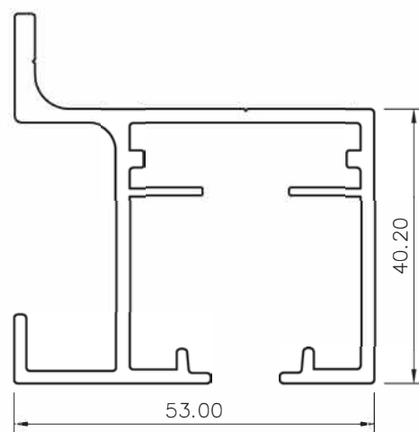
Ref. 35008***
