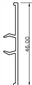
Ref. 35908**
