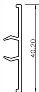
Ref. 35904**
