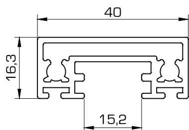
7610 Marco 40 mm
