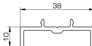
7621 Perfil interior industrial
