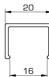
7600 "U" Pilastra industrial
