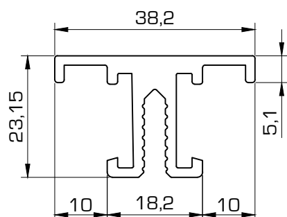
7620 Pilastra industrial
