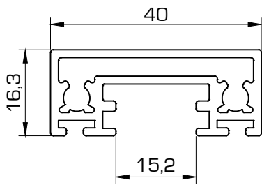
7610 Marco 40 mm
