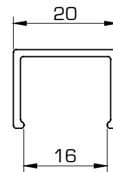
7600 "U" Pilastra industrial
