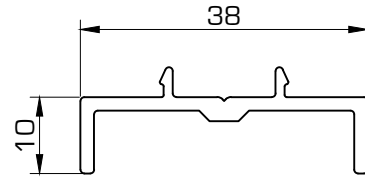
7621 Perfil interior industrial
