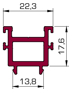
PO-223 Poliamida marco
